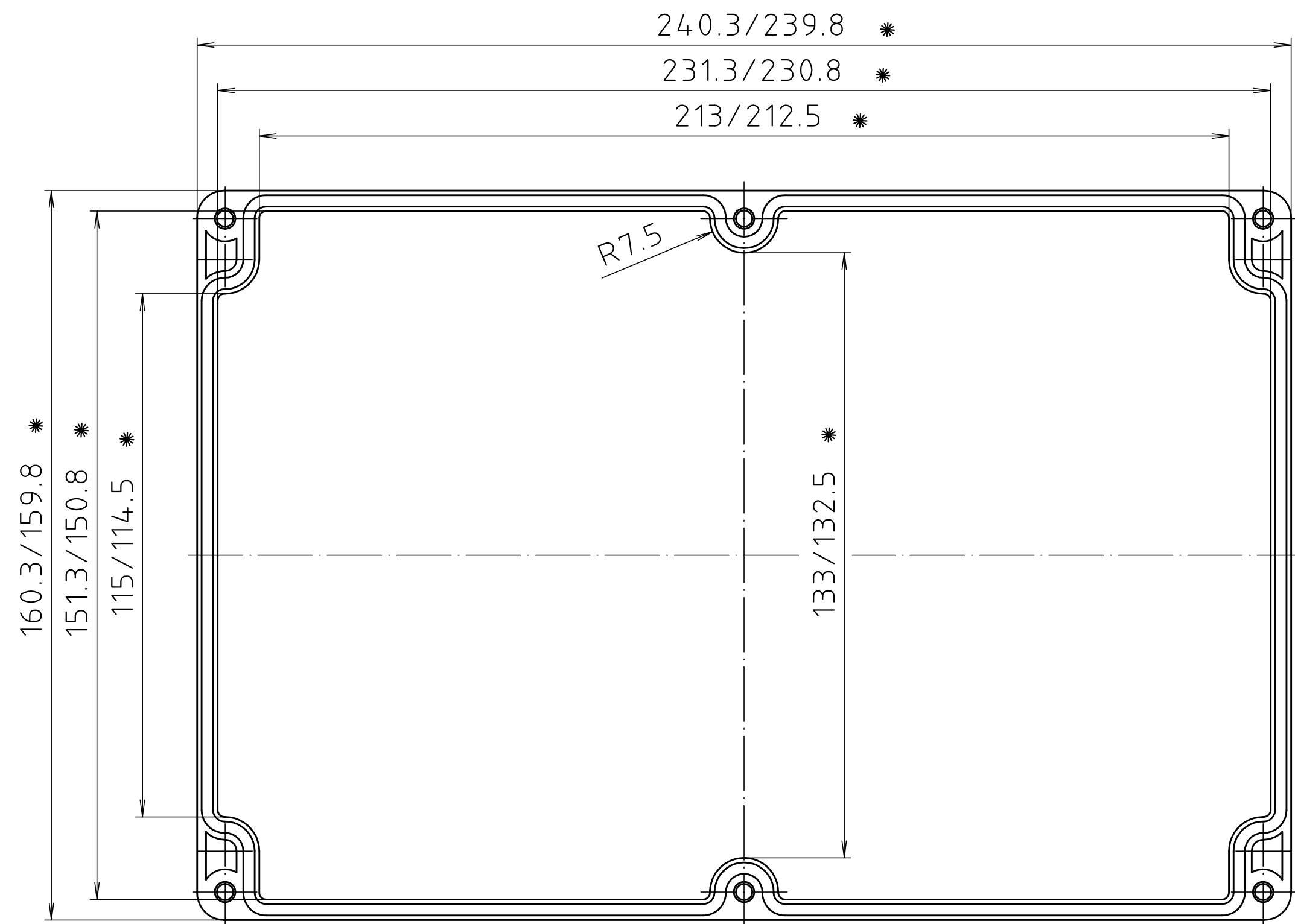
Deckel/lid
