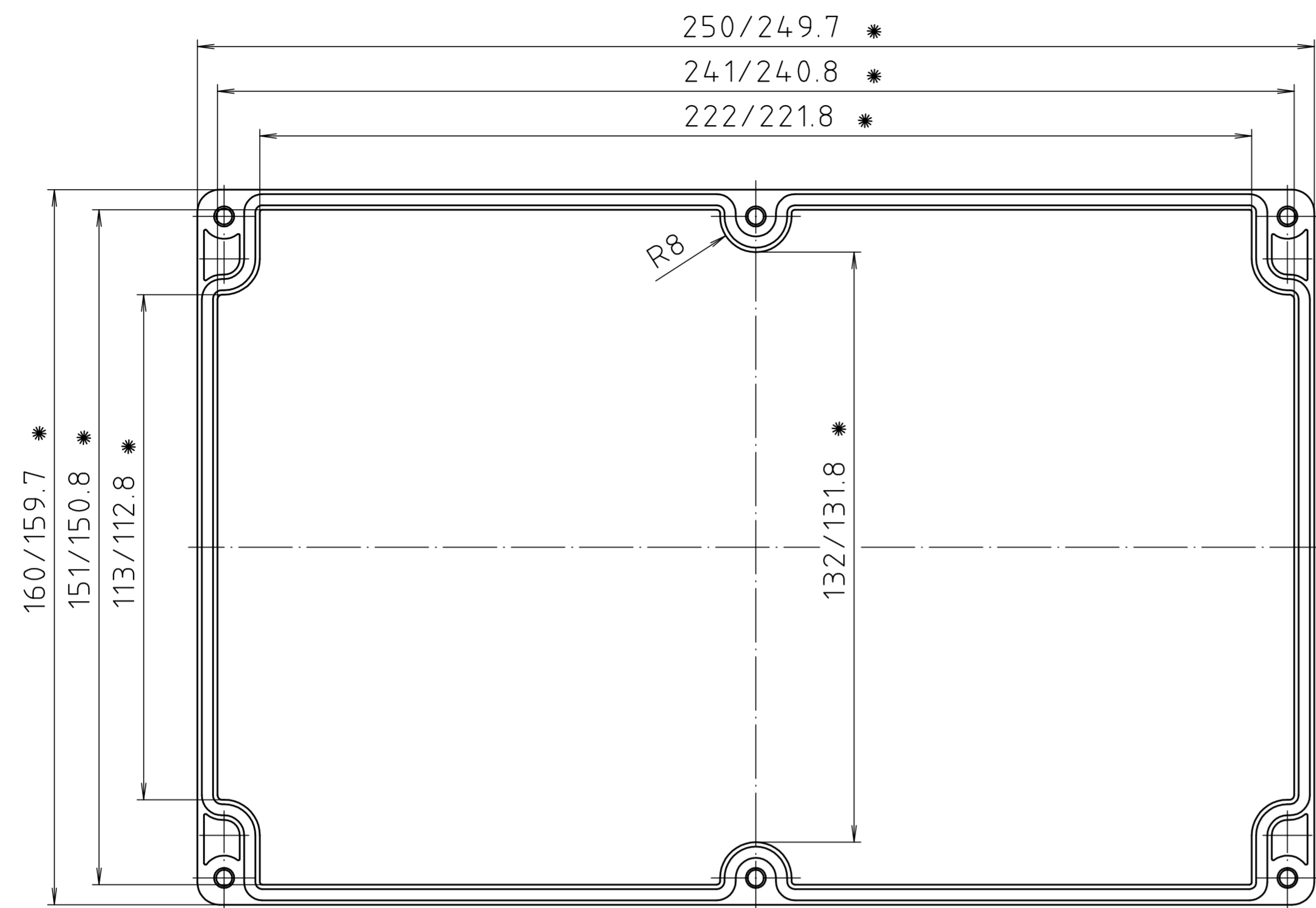
Deckel/lid
