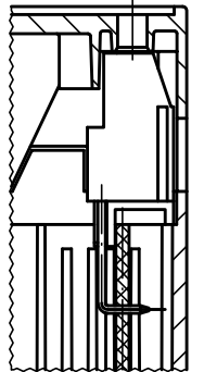
Anschlussklemme AK 700/. HB/ Connection terminals AK 700/. HB
