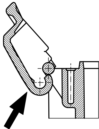
B SC HB-E Montagerichtung B SC HB-E mounting direction
